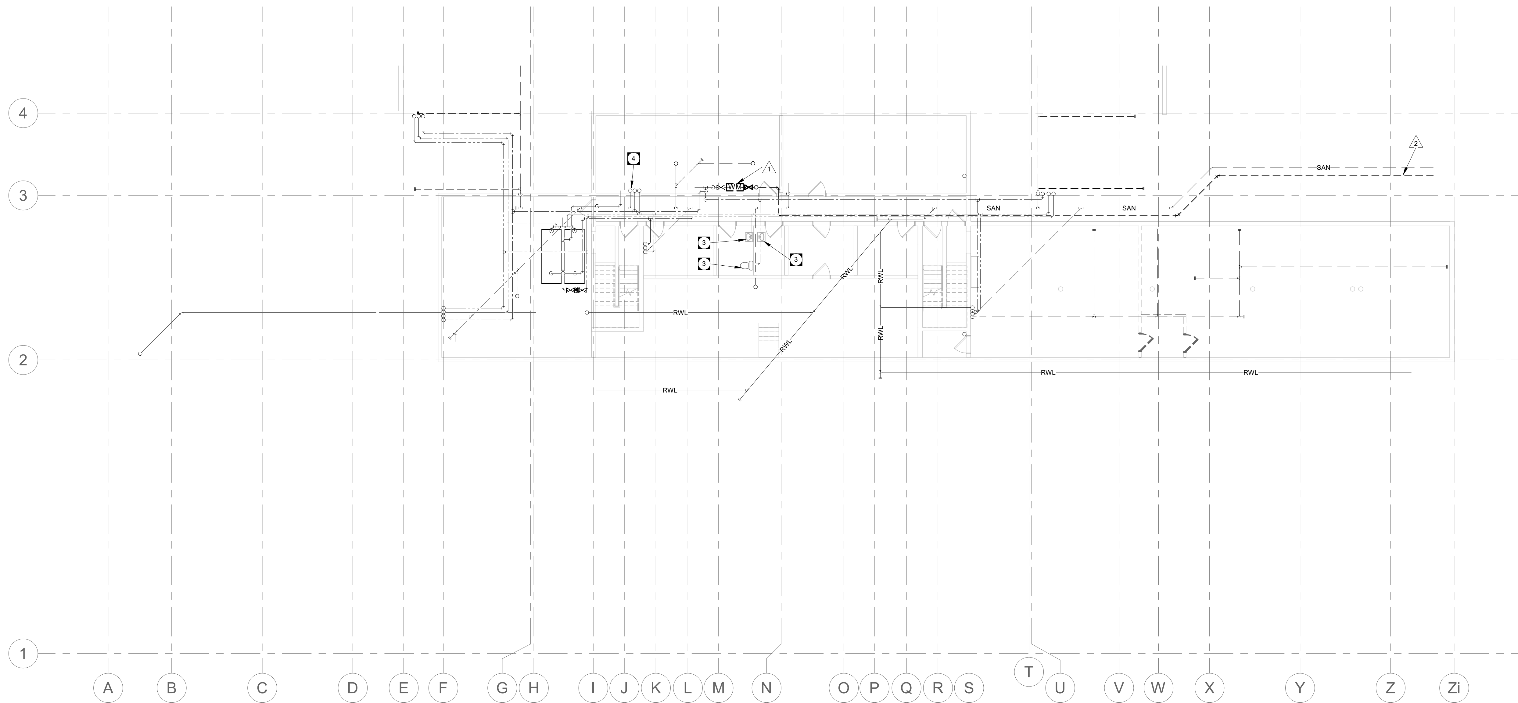
BASEMENT - PLUMBING DEMOLITION 1 3/32" = 1'-0" MP2.0
